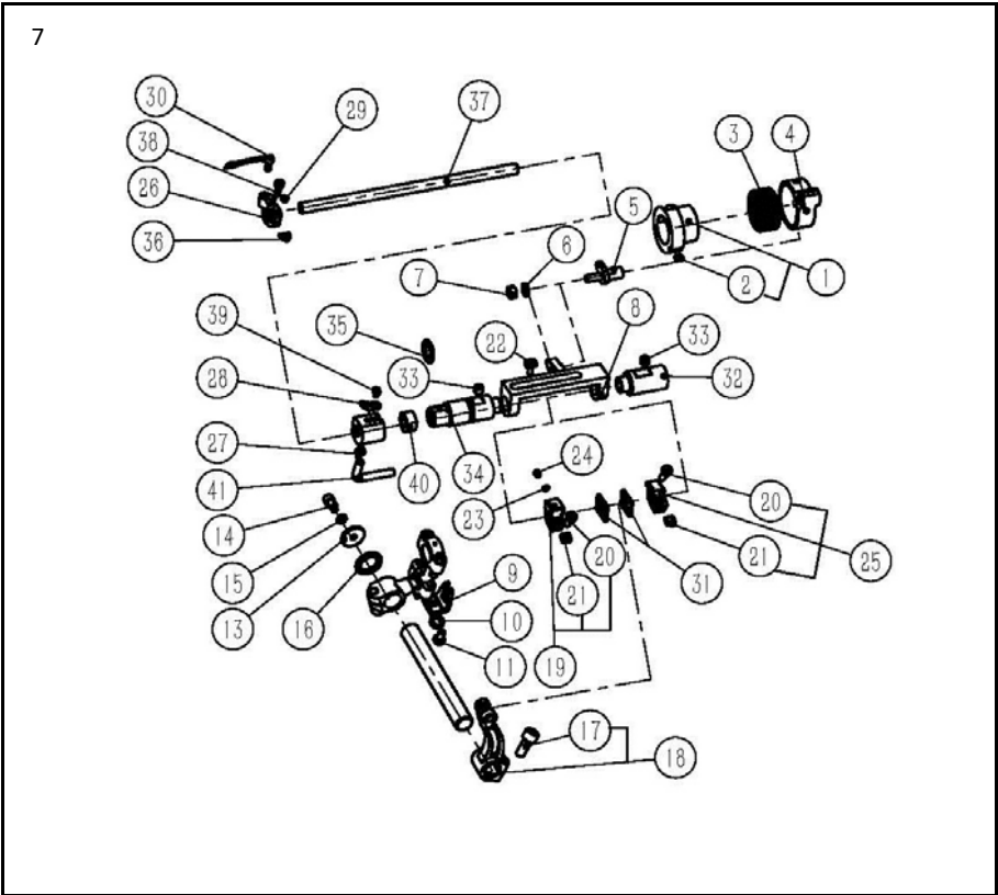
七、弯针部件/Needle guard assemblies
