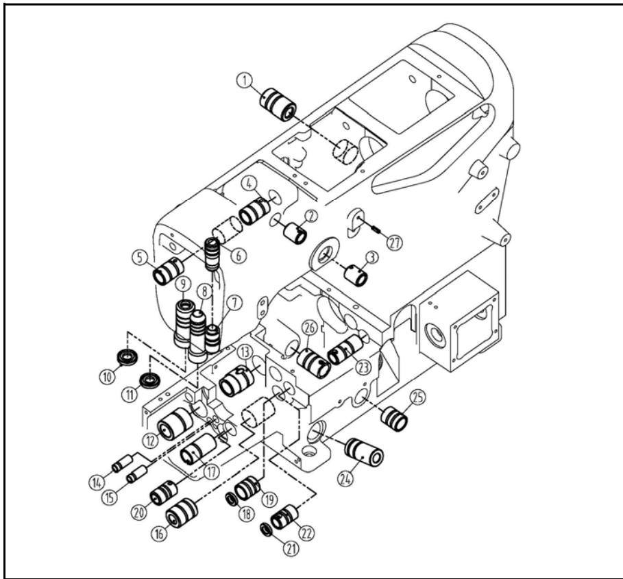
套筒部件/Bushing assemblies
