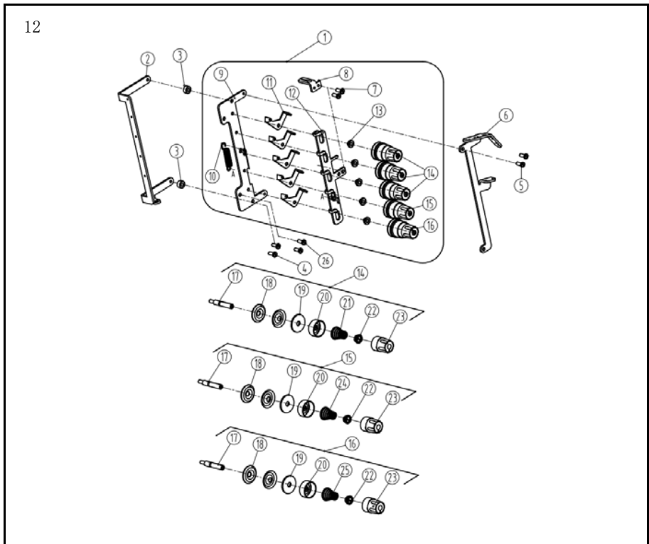
十二、松线部件(一)/Thread loosening assemblies (one)
