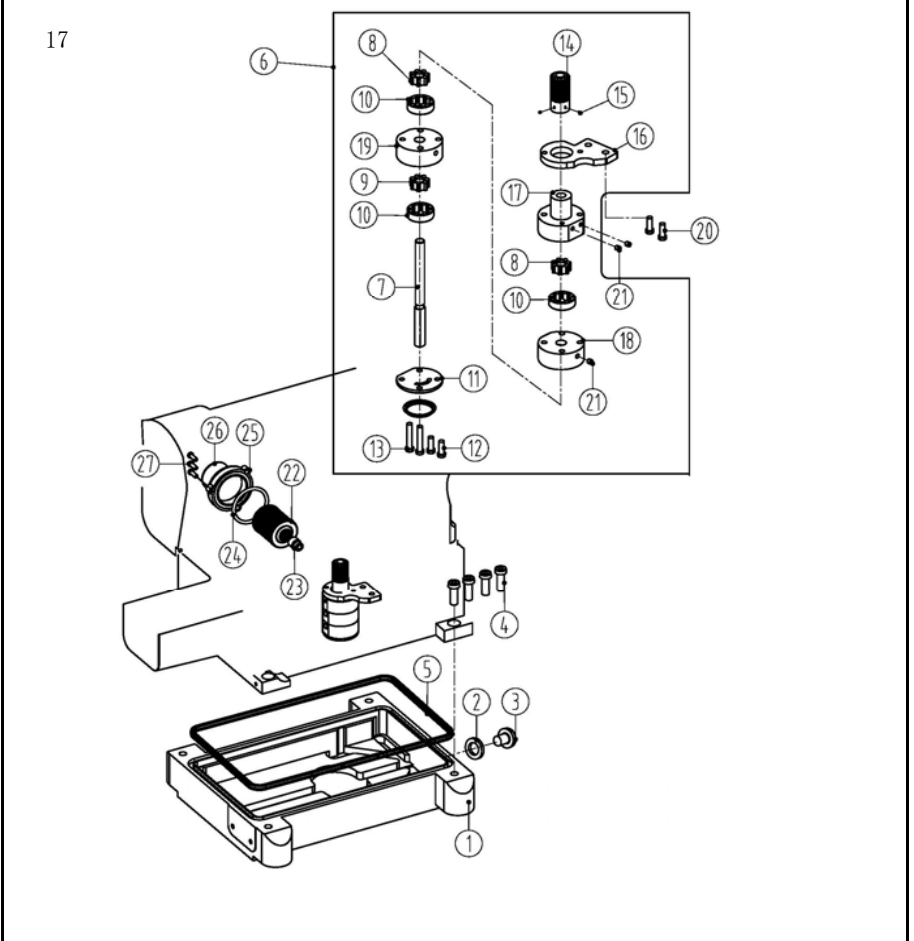
十七、油泵部件/Oil pump assemblies
