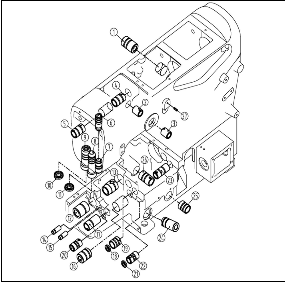
套筒部件/Bushing assemblies
