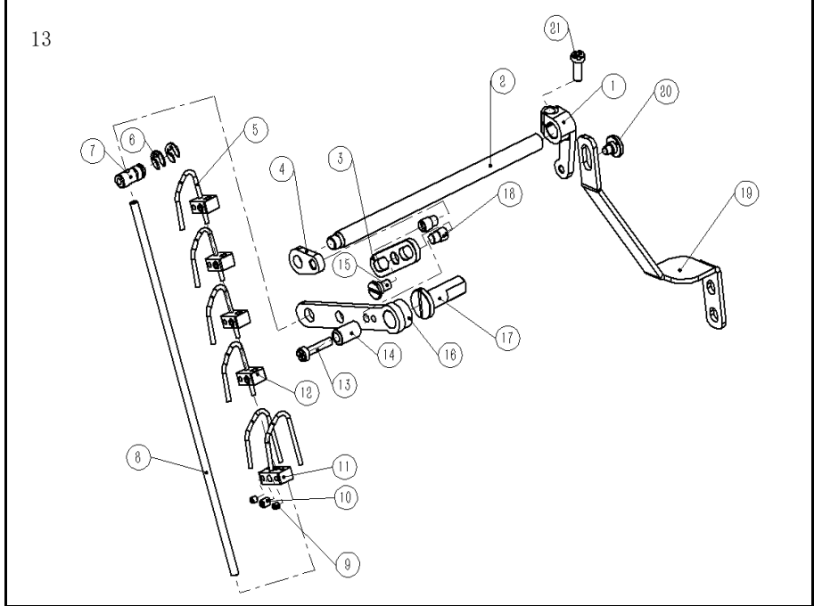
十三、松线部件(二)/Thread loosening assemblies (two)
