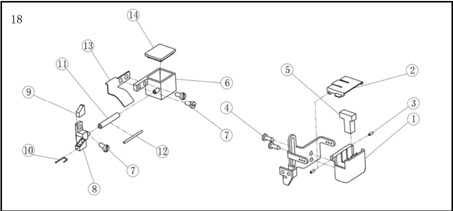
十八、硅油盒装置部件/Silicon oil delice assemblies
