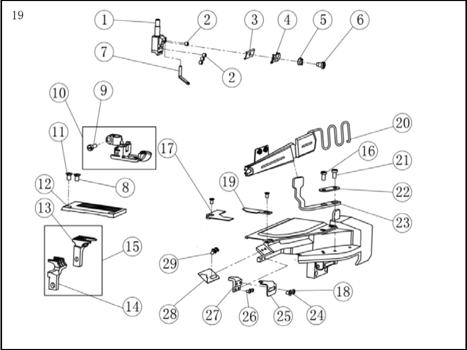
十九、针位组专用件部件/Gauge set specific parts
