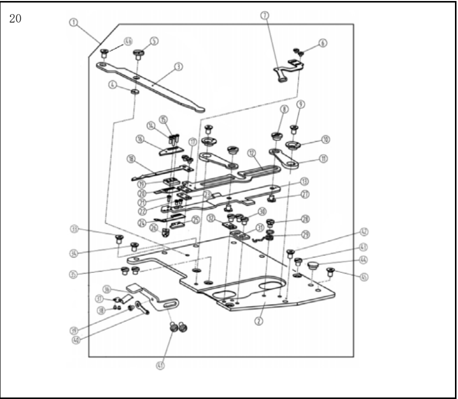
二十、下剪线部件/Knife holder assemblies
