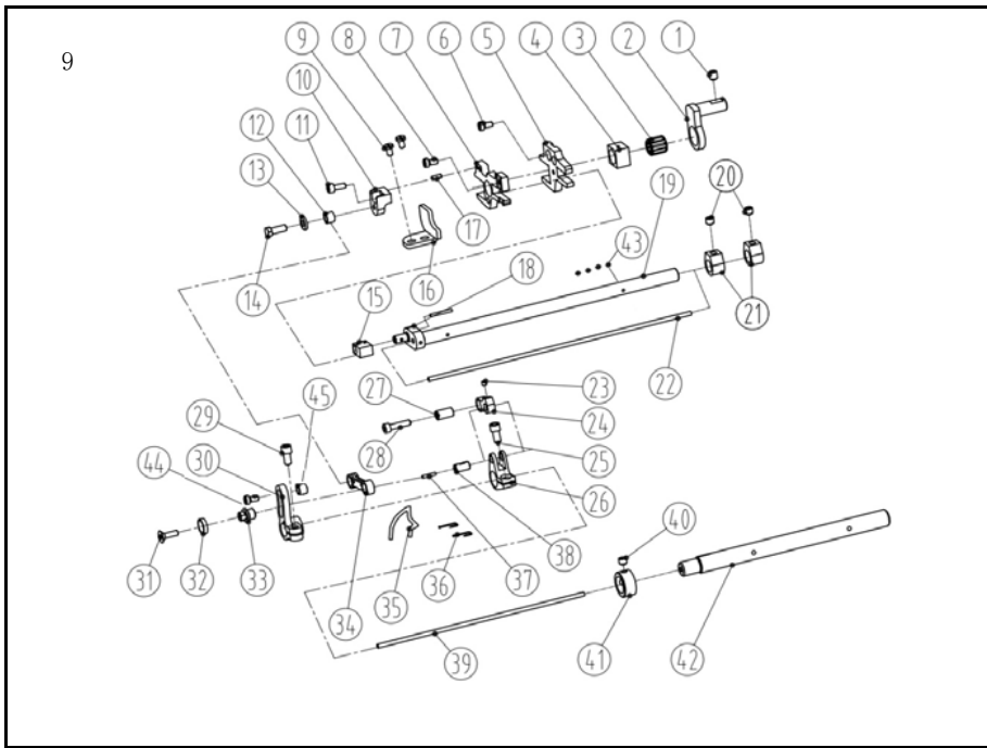
九、送布部件/Need mechanism
