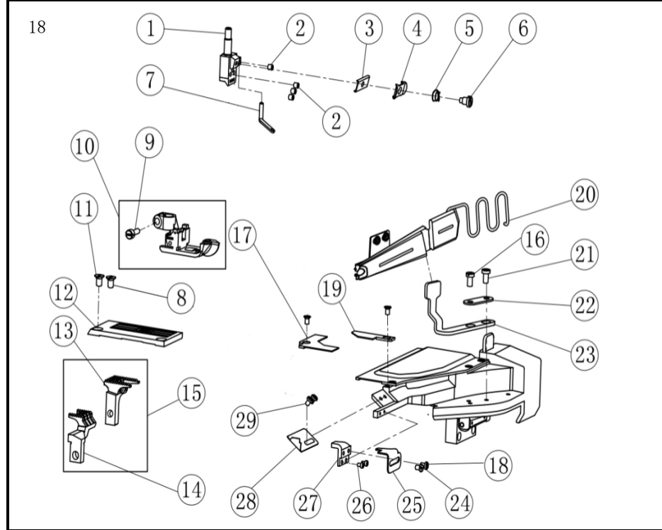
十八、针位组专用件部件/Gauge set specific parts
