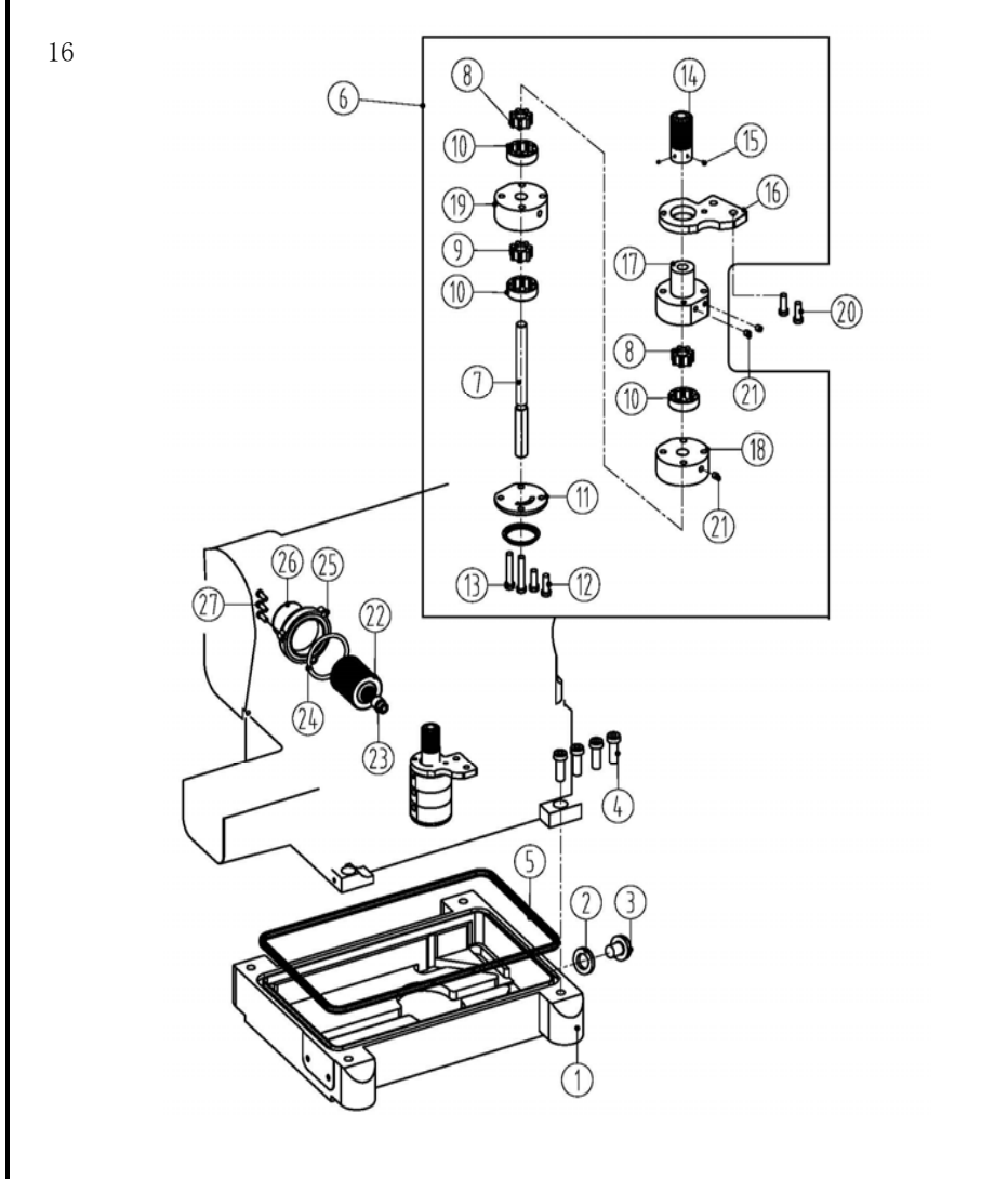
十八、针位组专用件部件/Gauge set specific parts
