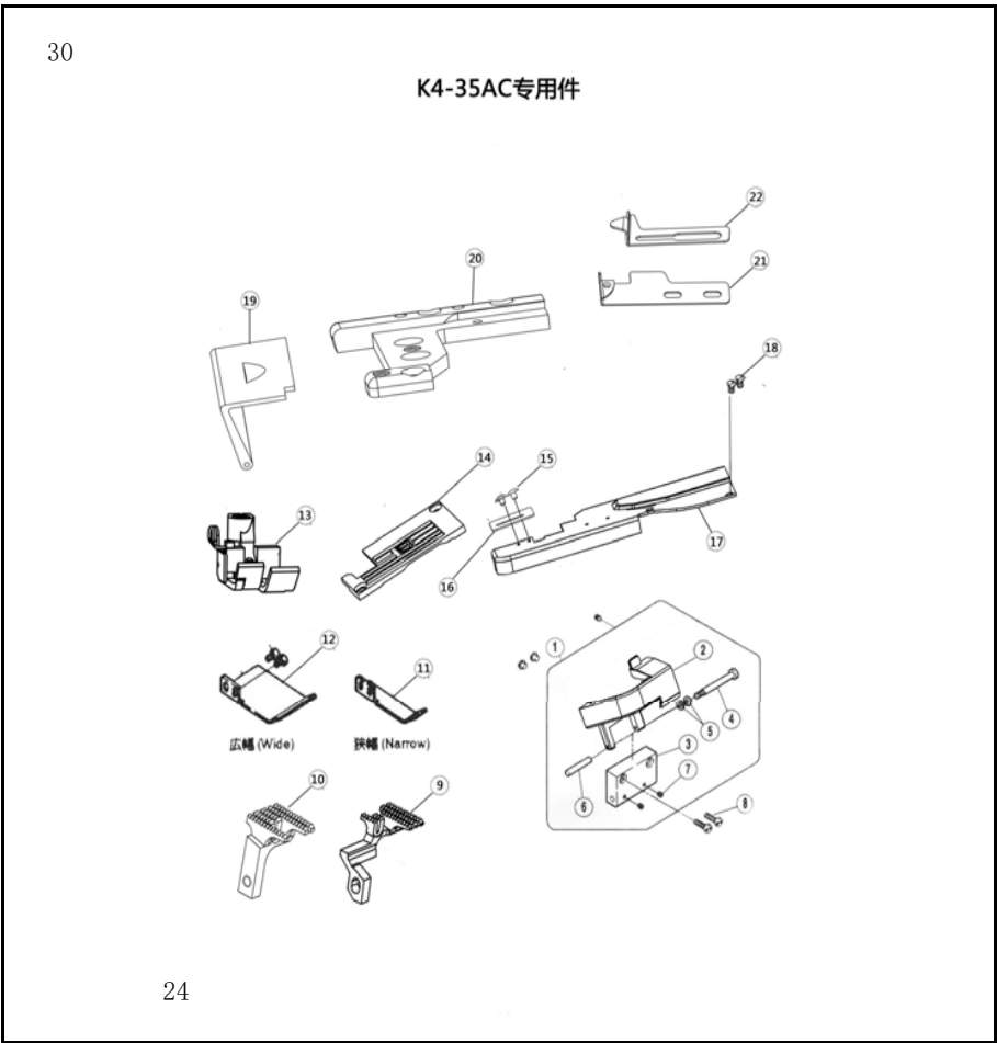
三十、35AC专用件/35ACFT device
