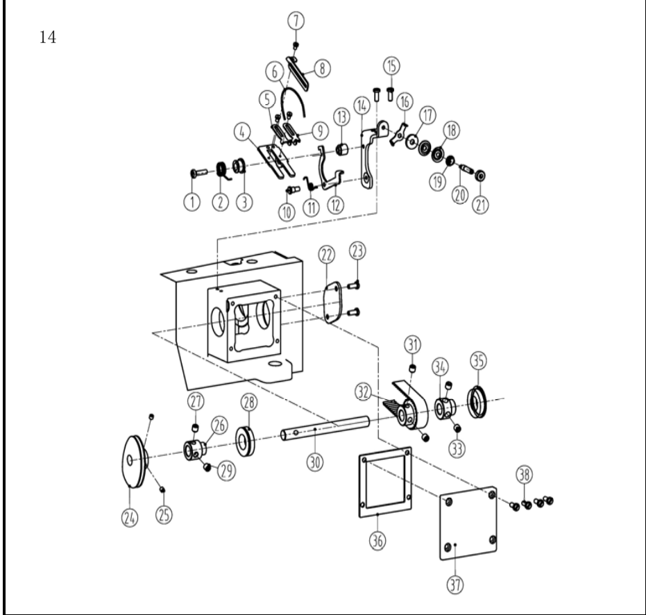
十四、打线凸轮部件/Cam assesblies
