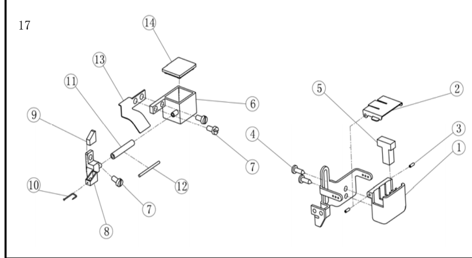
十七、硅油盒装置部件/Silicon oil delice assemblies
