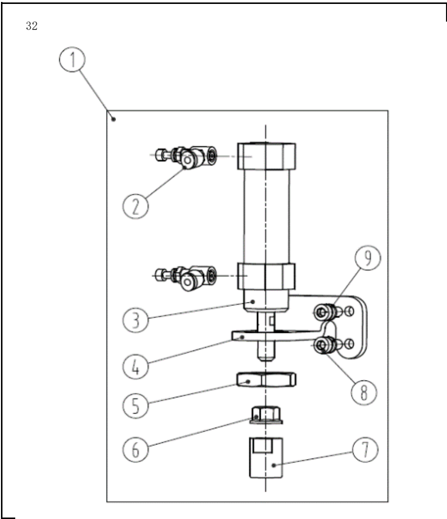
三十三、上剪线部件/Top shear unit
