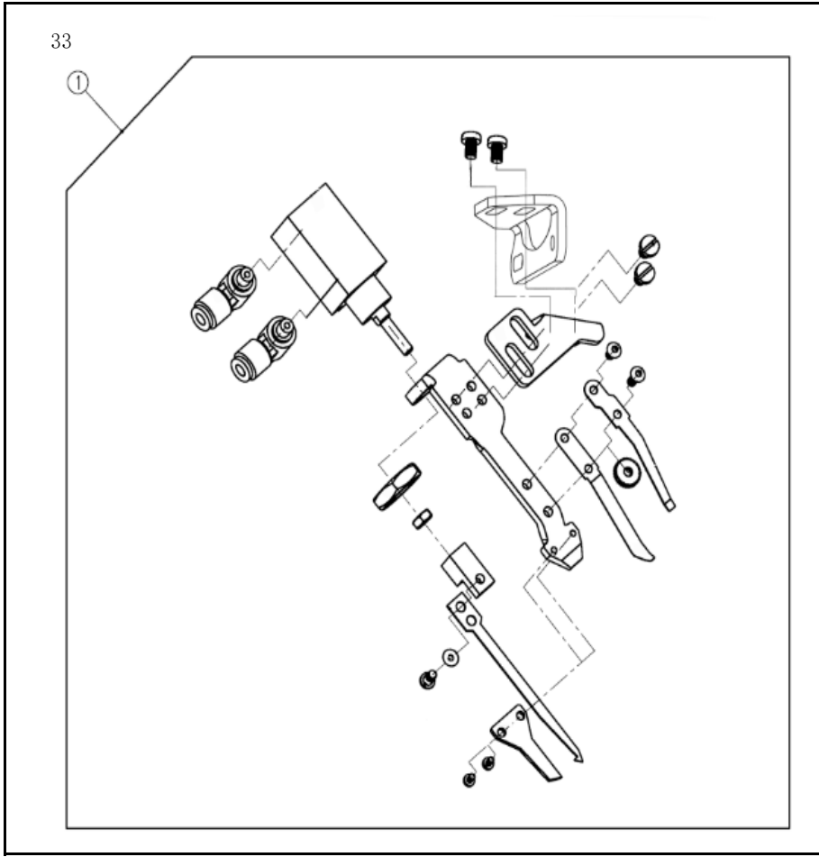
三十三、上剪线部件/Top shear unit
