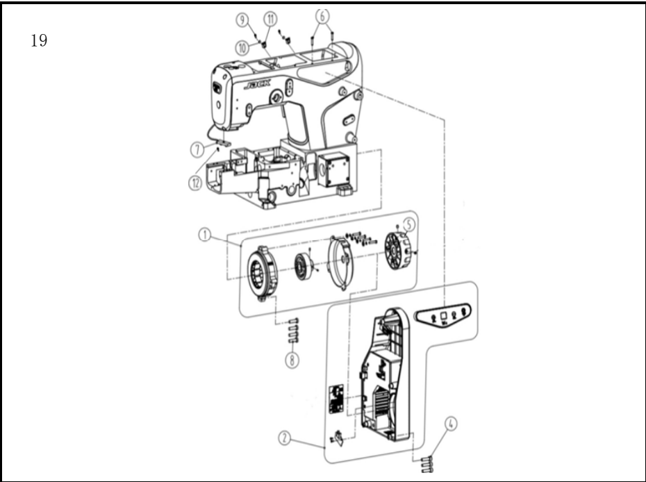
十九、电控部件/Electronic control assemblies
