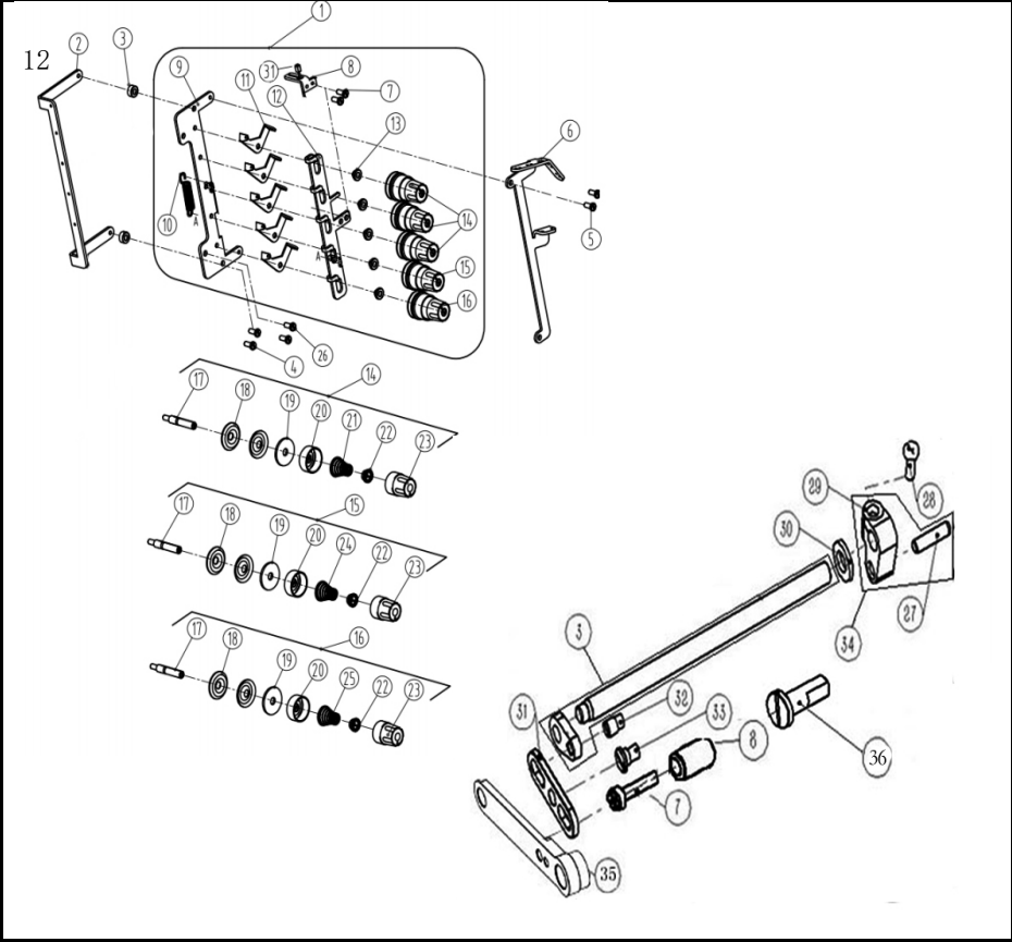
十二、松线部件/Thread loosing assemblies (one)
